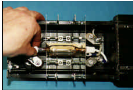
The P2 incorporates universal lamp holders to accept any type of lamp end fitting.
